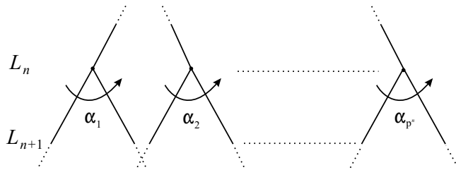
FIGURE 1. A part of the portrait of an automorphism f \in \text{Aut } T_p(v) .
