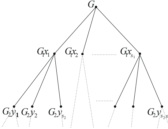
FIGURE 2. Construction of a coset tree T(\Sigma) .
