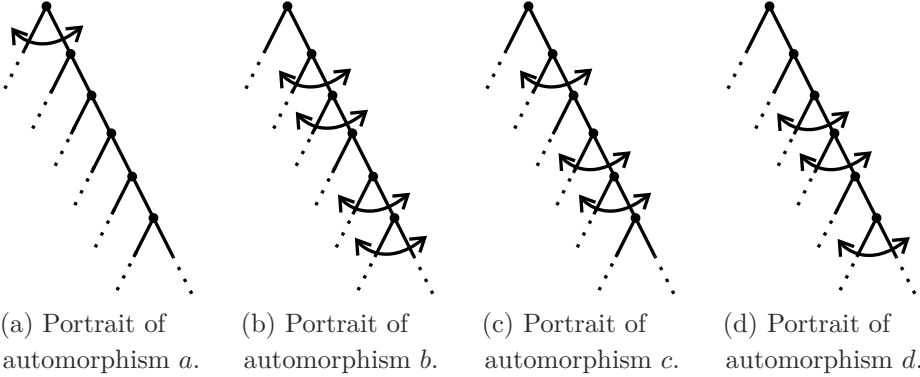
FIGURE 3. Portraits of generators of the first Grigorchuk group.
